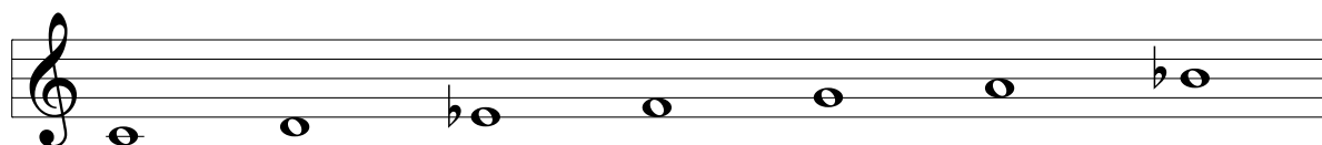
C_Blues scale
